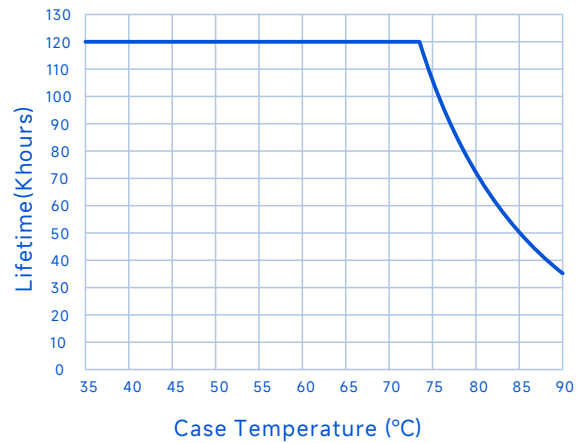
Lifespan vs. Case Temperature
